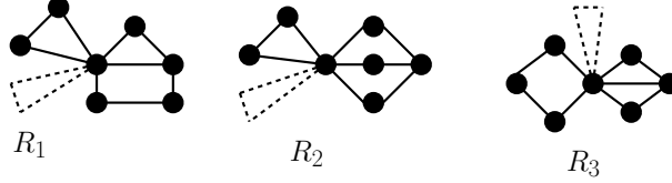
Fig. 3: All possible realizations of \varepsilon = (2a - 1)^1 3^1 2^{2a-1} . In realizations R_1 and R_2 , a - 2 triangles are attached to a vertex of degree 3 in a realization of 33222. In realization R_3 , a - 3 triangles and a single C_4 are attached to a dominating vertex in the diamond.
