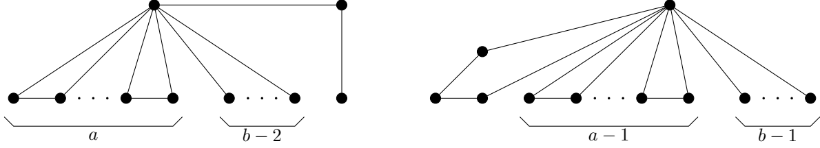
Fig. 2: The two realizations of (b + 2a - 1)^1 2^{2a+1} 1^{b-1} .
