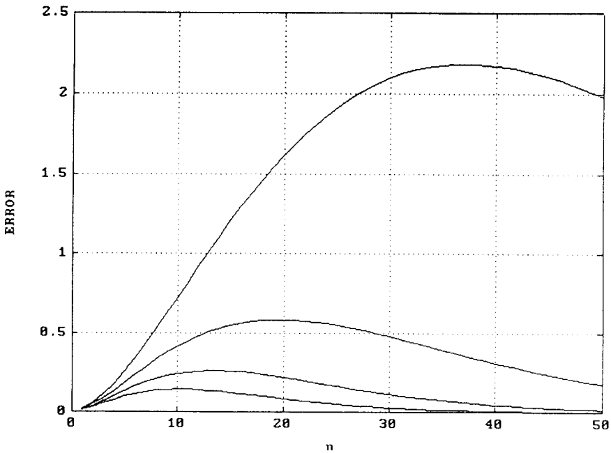
Figure 4. Error due to interpolation ( r_1 = 5\%, 10\%, 15\%, 20\% ; d = 1\% )
